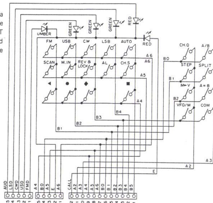
Fig. 6 Keyboard ass'y schematic diagram
