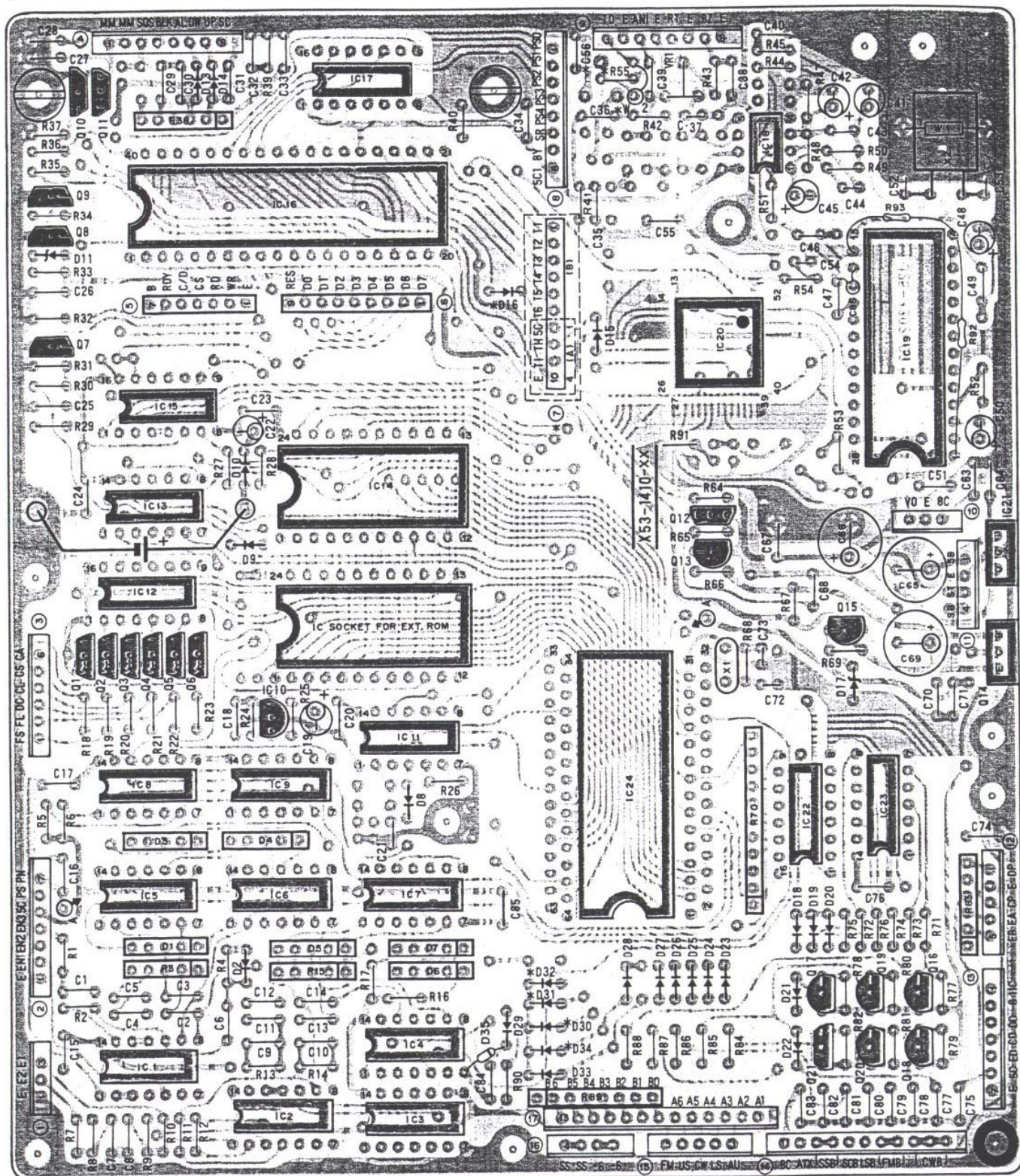
CONTROL UNIT (X53-1410-XX) Component side view (-12: TS-811 K -22: TS-811 M,X -52: TS-811 T -62: TS-811 W)
