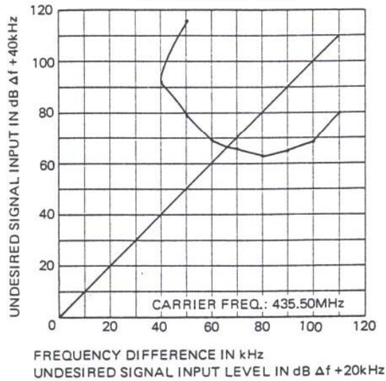
INTER MODULATION
