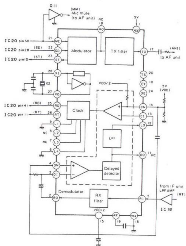
Fig. 10 Modem IC MN6127A block diagram (Control unit IC19)
