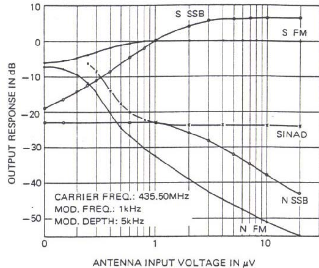
RX SENSITIVITY
