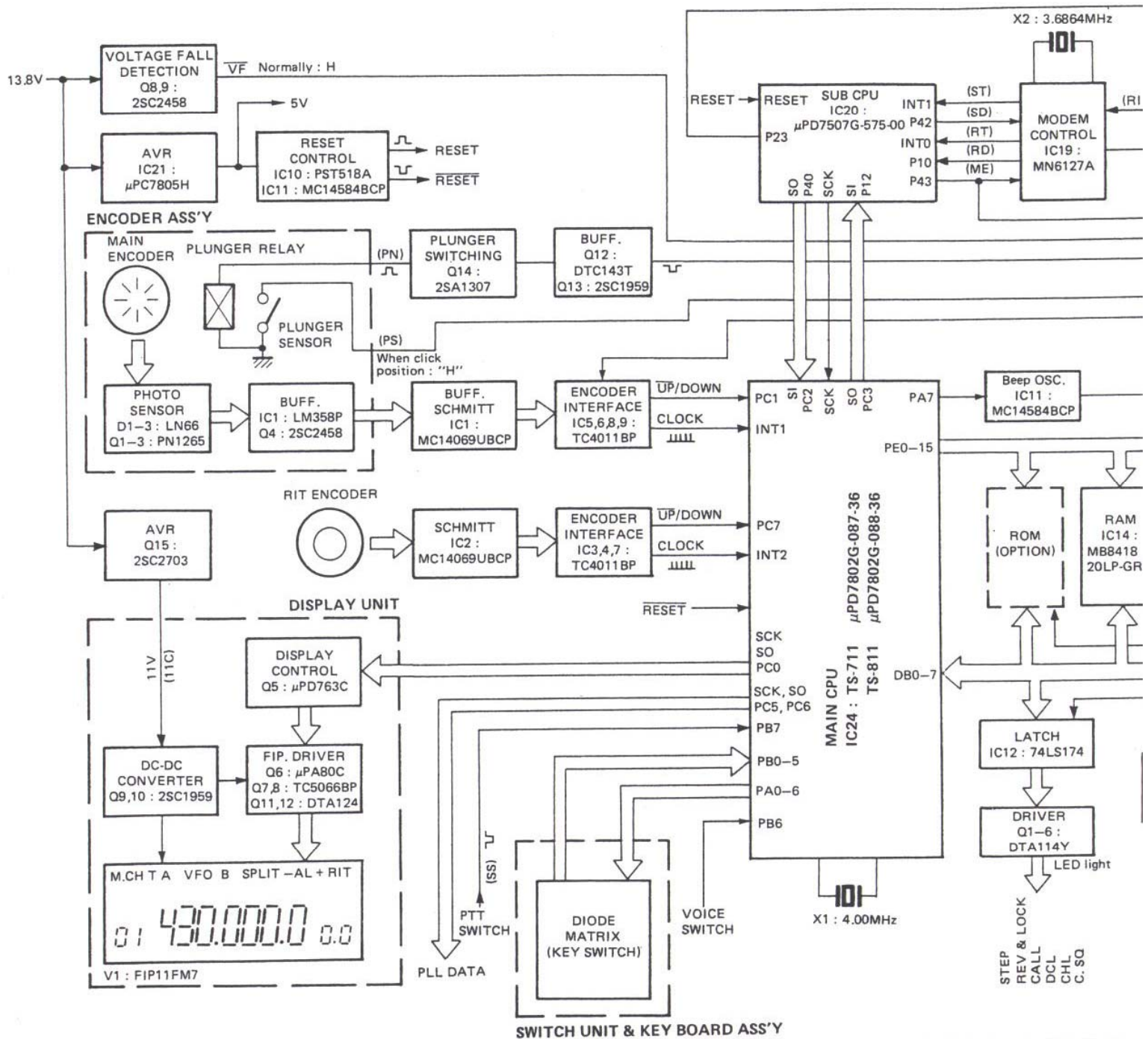
Fig. 5 Digital control block diagram
