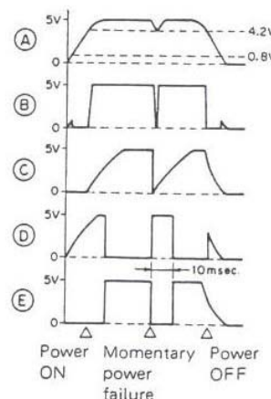
Fig. 11 Reset circuit and waveforms at respective points
